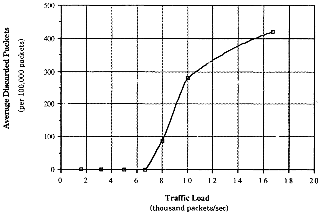
Graph 2. Average Discarded Packets vs Traffic Load (ETHERNET)
