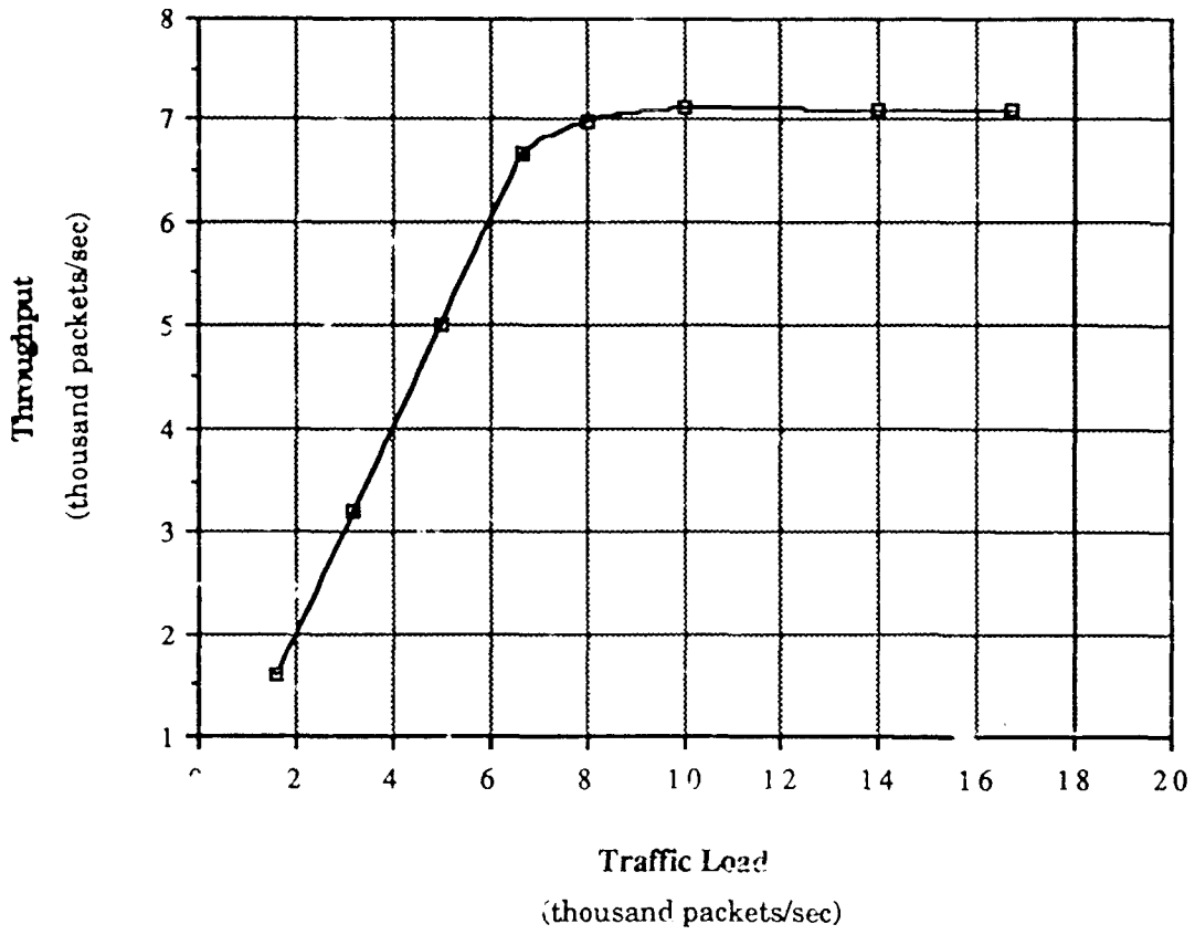
Graph 1. Throughput vs Traffic Load (ETHERNET)
